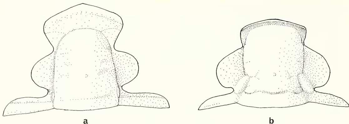
TEXT-FIG. 15. Cranidia of additional taxa here included in Asaphacea, showing diagnostic glabellar structure (cf. text-fig. 11). a , small cranidium of Haniwooides (Upper Cambrian, Australia) (after Shergold 1980, pl. 4), \times 8 . b , Macropyge , type species Macropyge chermi (Tremadoc) (new restoration), \times 4 .
